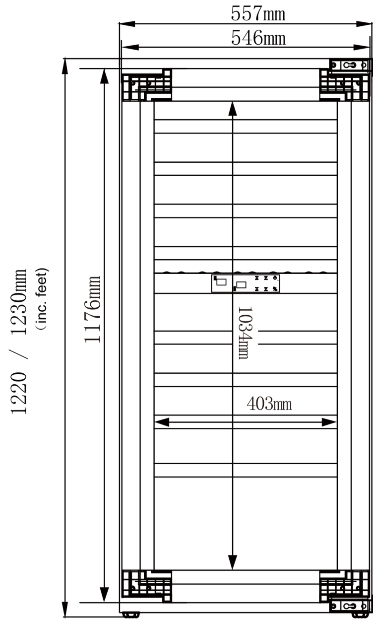
Front View
